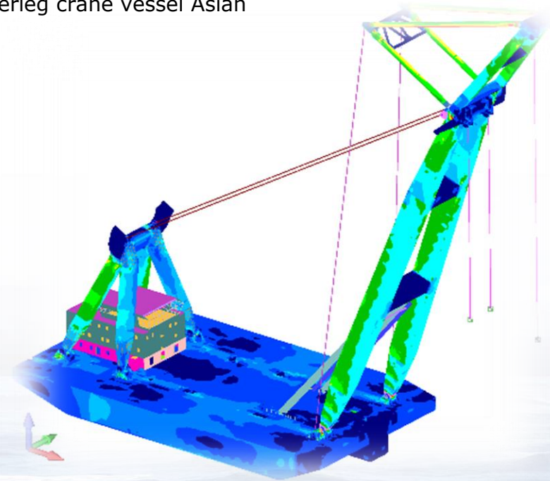
The FEM model of the “new” Asian Hercules
